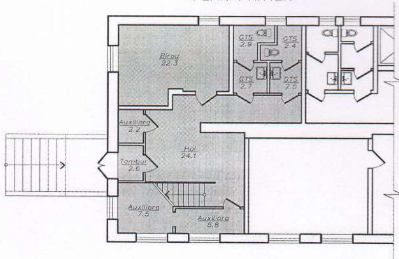
PLAN PARTER
